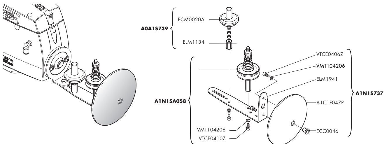
Disk tensioner for pneumatic threading with waxing unit
